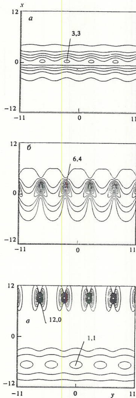
FIG. 1. The birth of 2D soliton chain as a result of the plane soliton instability described by Eq. (2.6) for M=1 : a— t=0 ; b— t=10 ; c— t=20 .
