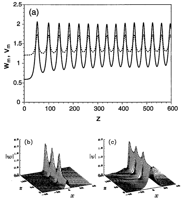
FIG. 3. Characteristic evolution of the unstable solitons for the case \sigma = 2 , \alpha = 0.05 , and \omega(0) > 0 . (a) Evolution of the soliton amplitudes w_m \equiv |w(0, z)| and v_m \equiv |v(0, z)| for the fundamental (solid curve) and second (dashed curve) harmonics. (b), (c) Propagation of the soliton components w and v , respectively.
