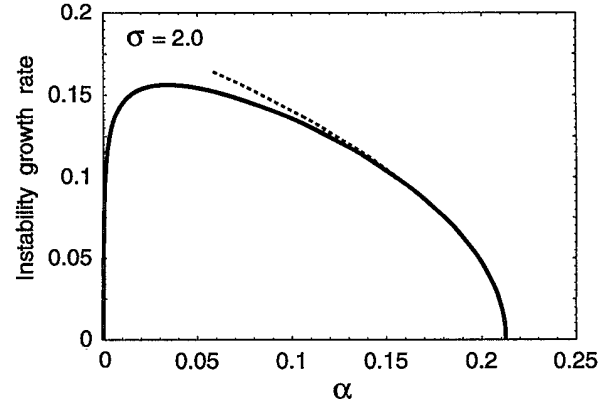
FIG. 2. Growth rate of linear instability at \sigma = 2 calculated numerically (solid curve). The analytical asymptotic (7) is shown by a dashed line.
