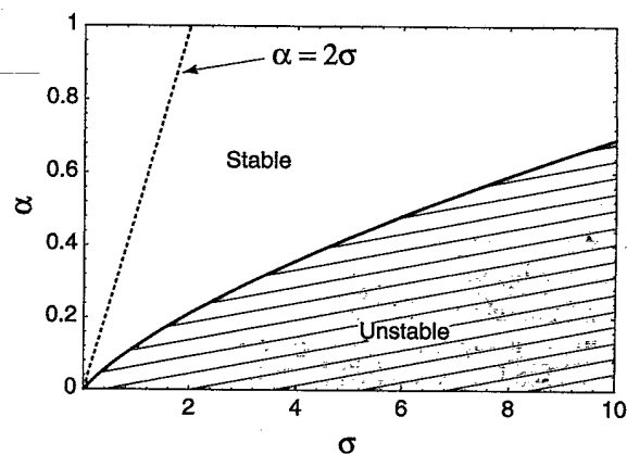
FIG. 1. Region of linear instability of two-wave solitons on the parameter plane ( \alpha, \sigma ). The dashed line \alpha = 2\sigma corresponds to the phase-matched interaction between the harmonics at \Delta k = 0 .
