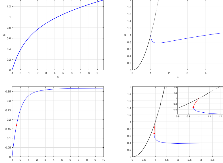
Fig. 4 Left: the dependence of b versus c for \alpha = 0.6 (top) and \alpha = 0.5 (bottom). Right: the dependence of \mu versus \omega = c for \alpha = 0.6 (top) and \alpha = 0.5 (bottom). Reproduced from [35].
