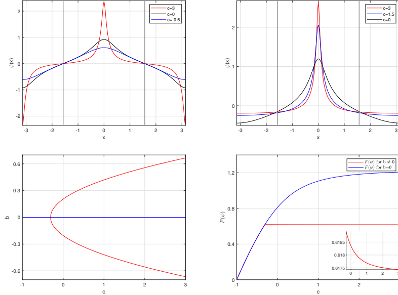
Fig. 5 Periodic solutions of the variational problem (33) with m = 0 for \alpha = 1 . Top: Profiles of \phi_c with b = 0 (left) and with b = b(c) \neq 0 (right) for three different values of c . Bottom left: Dependence of b versus c showing the pitchfork bifurcation point c_0 . Bottom right: Dependence of the momentum \mu = F(\phi_c) versus c . Reproduced from [36].
