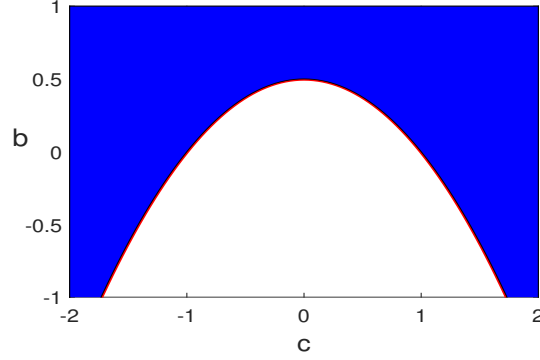
Fig. 1 The existence region on the parameter plane (c, b) for the single-lobe periodic solutions of the stationary equation (9) obtained with (10) and (11) for \omega \geq 1 .
