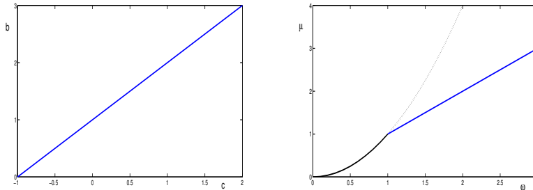
Fig. 3 The dependence of b versus c (left) and \mu versus \omega = c (right) for \alpha = 1 . Reproduced from [35].
