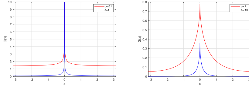
Fig. 2 Profiles of G_c for specific values of c are plotted versus x on \mathbf{T} for \alpha = 0.5 (left) and \alpha = 1.5 (right). Reproduced from [29].
