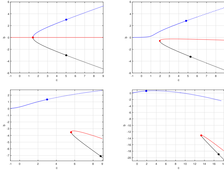
Fig. 6 Three solution families on the (b, c) diagram for fixed values of m : m = 0 (top left), m = 0.01 (top right), m = 0.1 (bottom left), and m = 0.2 (bottom right). Reproduced from [30].
