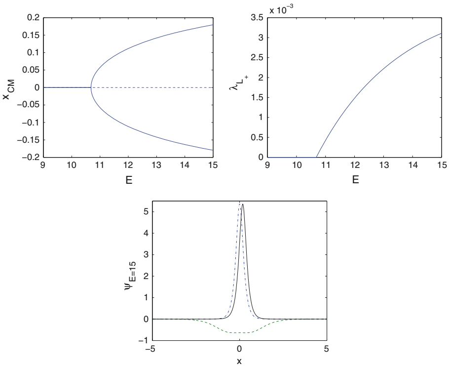
Fig. 2. The top left panel shows the pitchfork bifurcation of asymmetric states for s = 0.7 > s_* and p = 1 . Two asymmetric ( x_{CM} \neq 0 ) states emerge for E > E_* \approx 10.68 . The second eigenvalue of L_+ for such asymmetric states is positive as shown in the top right panel. The bottom panel shows symmetric and asymmetric states versus x for E = 15
