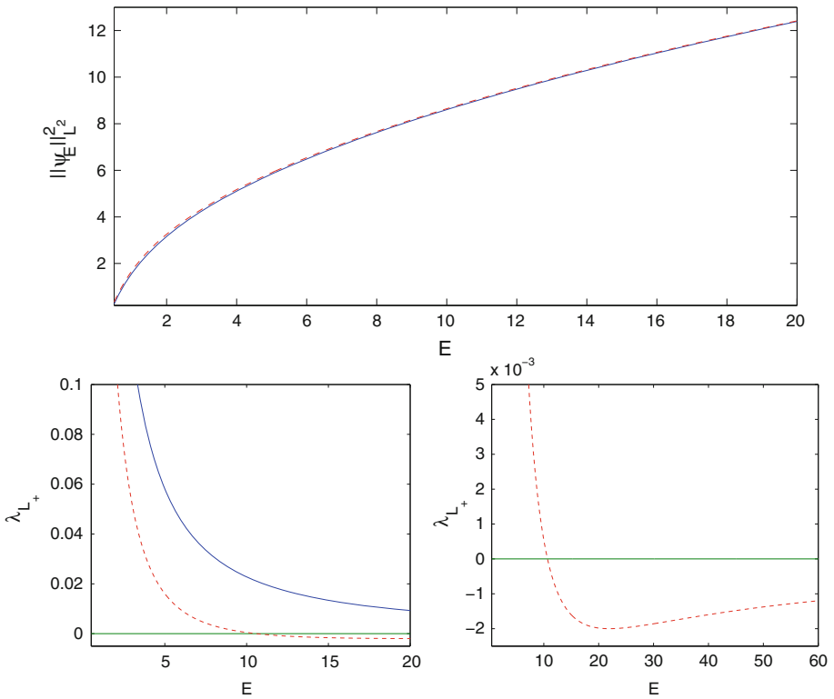
Fig. 1. The top panel shows the dependence of the squared L^2 norm of the symmetric state on the parameter E for p = 1 . The bottom left panel shows the trajectory of the second eigenvalue of L_+ for the cases of s = 0.6 < s_* (blue solid line) and s = 0.7 > s_* (red dashed line). The bottom right panel shows an expanded plot of the second case for considerably larger values of E
