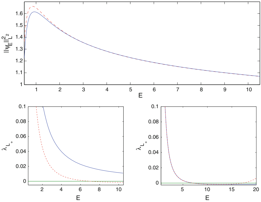
Fig. 3. The top and bottom left panels are similar to Fig. 1, but now for p = 3 . The blue solid line corresponds to the case of s = 0.6 < s_* , while the red dashed to s = 0.7 > s_* . The bottom right panel shows the importance of sufficiently fine discretization in resolving this second eigenvalue for large E . Here the red dashed line corresponds to a spatial grid spacing of \Delta x = 0.025 , while the solid blue line is obtained for \Delta x = 0.0125
