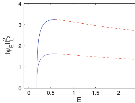
Fig. 4. The graph shows the dependence of the squared L^2 norm of the stationary states on the parameter E for p = 3 and s = 10 . The left most (blue solid) line are the anti-symmetric (excited) states emerging from zero at the second lowest eigenvalue E_1 = 0.191042 . Almost on top of it is the (blue solid) line of symmetric ground states emerging from zero at E_0 = 0.191046 . The latter bifurcates at E_* \approx E_0 into the dashed red line (symmetric states) and the right most blue solid line (asymmetric states). At E \approx 0.5908 the slope of the L^2 norm becomes negative for all branches. The solid lines denote linearly stable branches, while dashed ones denote unstable branches
