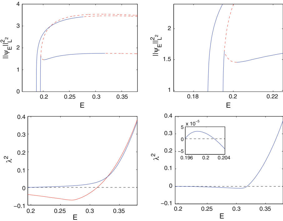
Fig. 5. The top panels show dependence of the squared L^2 norm of the stationary states on the parameter E for p = 5 , s = 4 , where the right panel is a blowup of the left panel. The leftmost branch is the anti-symmetric (excited) states and the other branch corresponds to the symmetric ground states which bifurcate into asymmetric states. The bottom panels show the squared eigenvalue of the linearization spectrum associated with the symmetric (left) and asymmetric (right) branches. The insert on the bottom right panel gives a blowup of the figure to illustrate instability of asymmetric states near the subcritical pitchfork bifurcation. The solid lines on the top panels denote linearly stable branches, while dashed ones denote unstable branches
