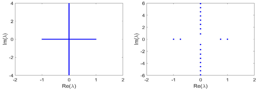
Fig. 1 Left: The Lax spectrum \Sigma_0 in L^2(\mathbb{R}) . Right: The union \Sigma_0^{(P)} \cup \Sigma_0^{(A)} of the Lax spectra in L^2_{\text{per}}(0, L) and L^2_{\text{antiper}}(0, L) for some L \in (\pi, 2\pi)
