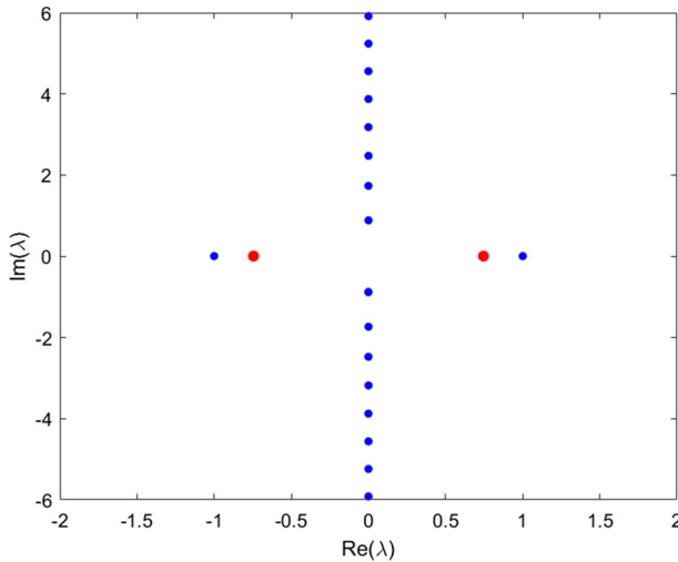
Fig. 2 The union \Sigma_{AB}^{(P)} \cup \Sigma_{AB}^{(A)} of the Lax spectra in L^2_{\text{per}}(0, L) and L^2_{\text{antiper}}(0, L) for AB. The red dots represent the eigenvalues \{+\lambda_0, -\lambda_0\} which are the only real eigenvalues in addition to \{+1, -1\} if L \in (\pi, 2\pi)
