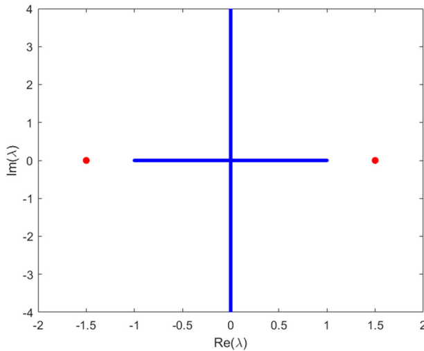
Fig. 3 The Lax spectrum \Sigma_{\text{KMB}} in L^2(\mathbb{R}) for KMB
